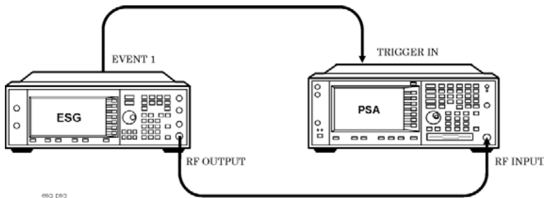
Figure 16-47 PSA Setup
