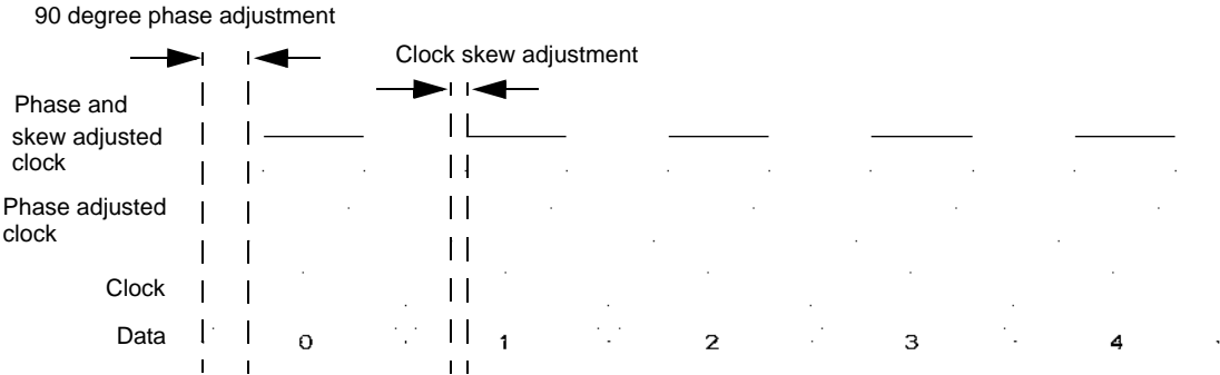
Figure 7-7 Clock Phase and Skew Adjustments
