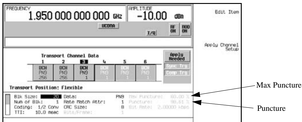
Figure 16-41 Excessive Puncturing
