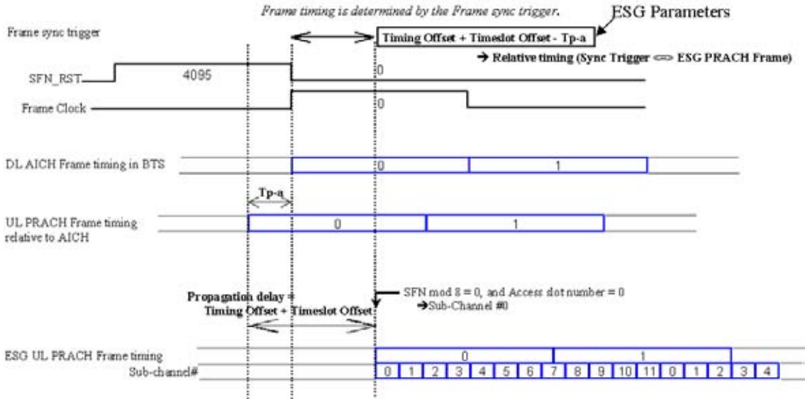
Figure 16-83 PRACH Synchronization - Frame Timing Alignment
