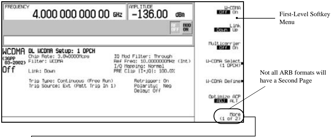
Figure 4-13 ARB Marker Location and Softkey Menus
