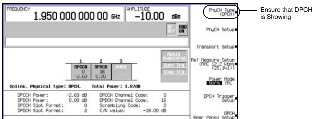
Figure 16-49 DPCCH is Selected
