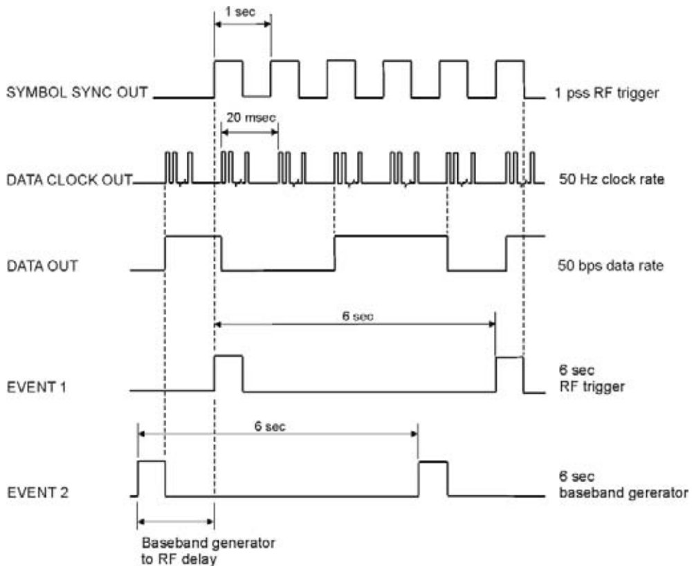
Figure 11-5 GPS Signals
