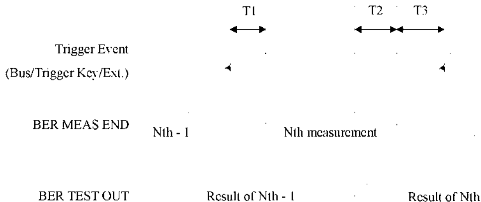
Figure 9-30 Testing Signal Definitions
