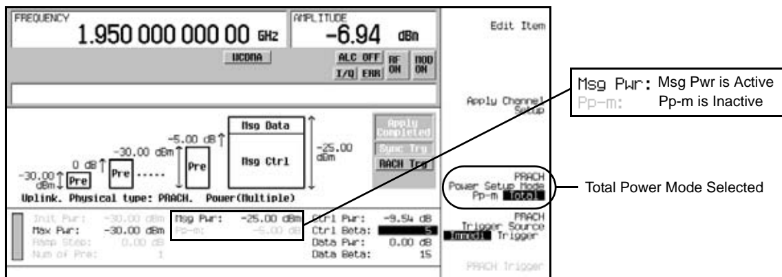
Figure 16-11 Total Mode Selection
