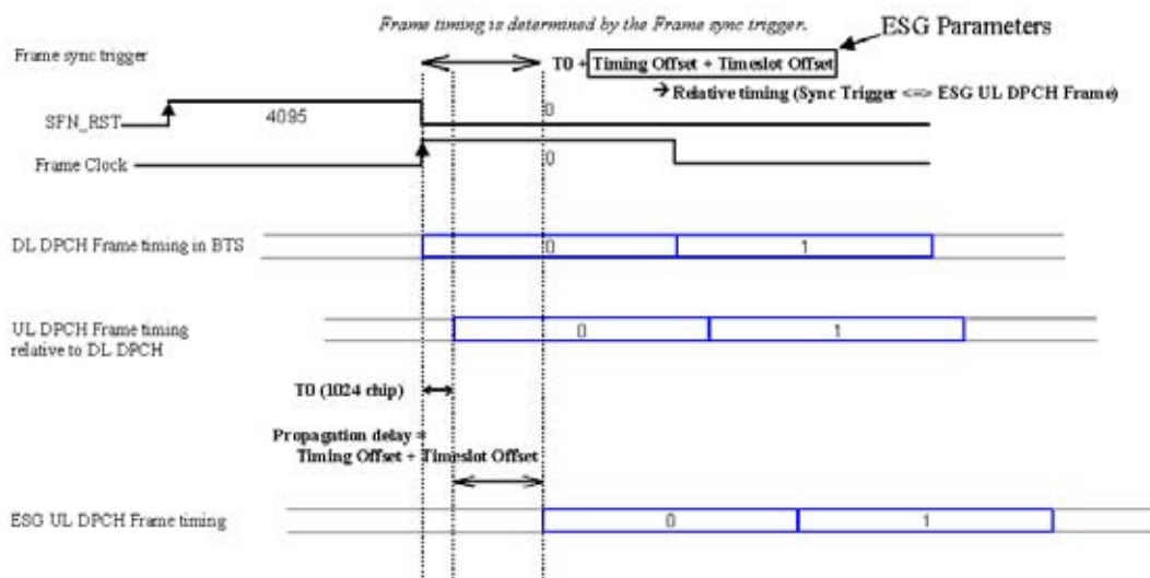
Figure 16-79 DPCCH Synchronization - Frame Timing Alignment
