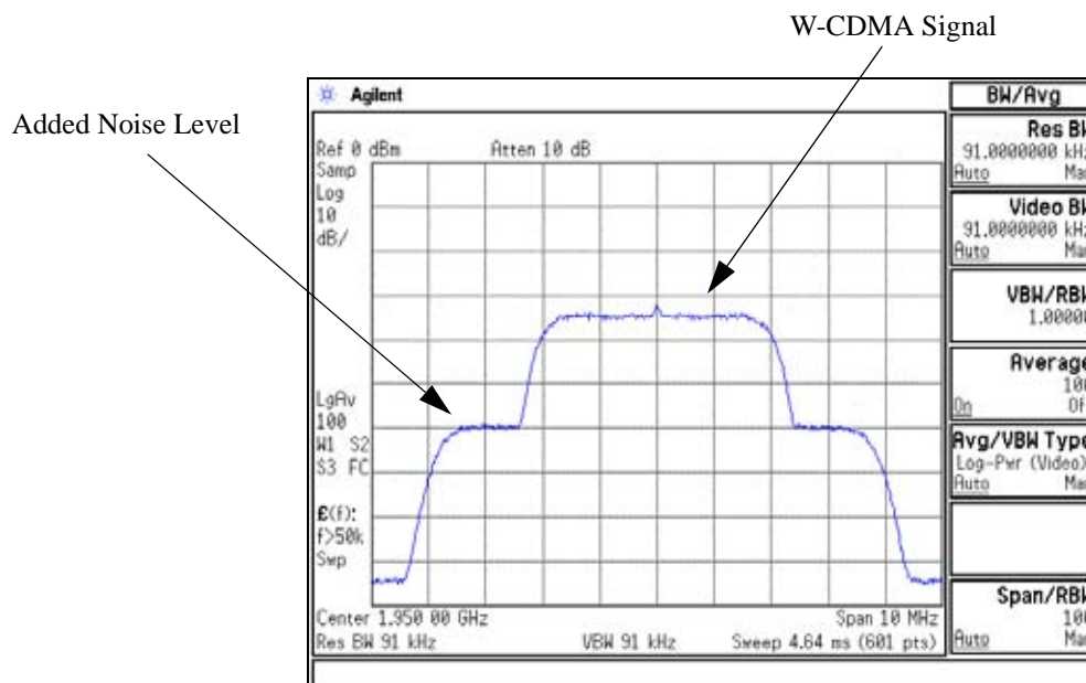
Figure 16-42 C/N Setting
