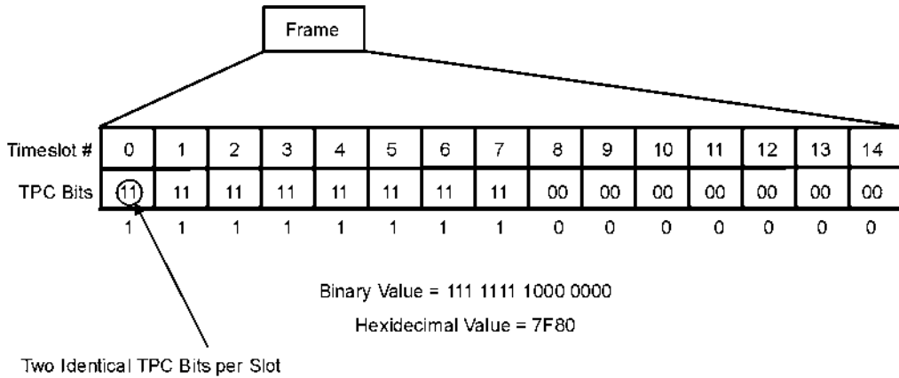
Figure 15-11 TPC Bits per Timeslot
