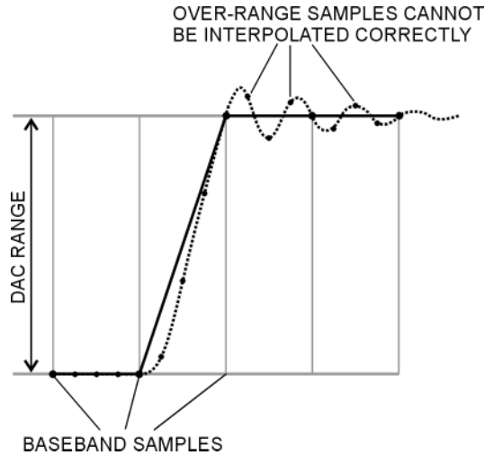
Figure 4-23 Waveform Overshoot
