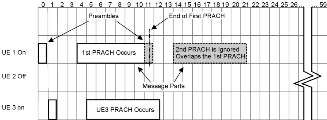
Figure 16-21 Transmitting PRACHs
