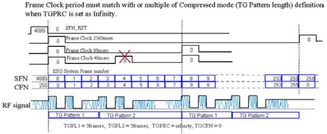
Figure 16-81 DPCH Synchronization - Frame Number Alignment for Continuous (Infinity) Compressed Mode
