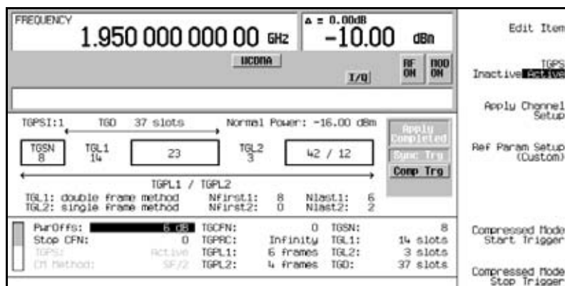
Figure 16-52 Compressed Mode Setup
