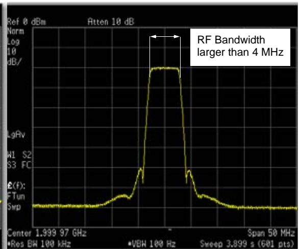
2.1 MHz Filter
