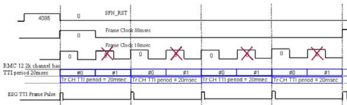
Figure 16-80 DPCCH Synchronization - Frame Number Alignment
