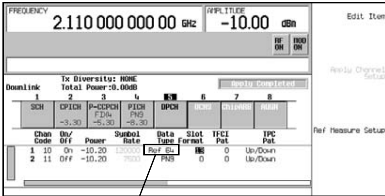
Figure 17-16 64 kbps RMC Selected
